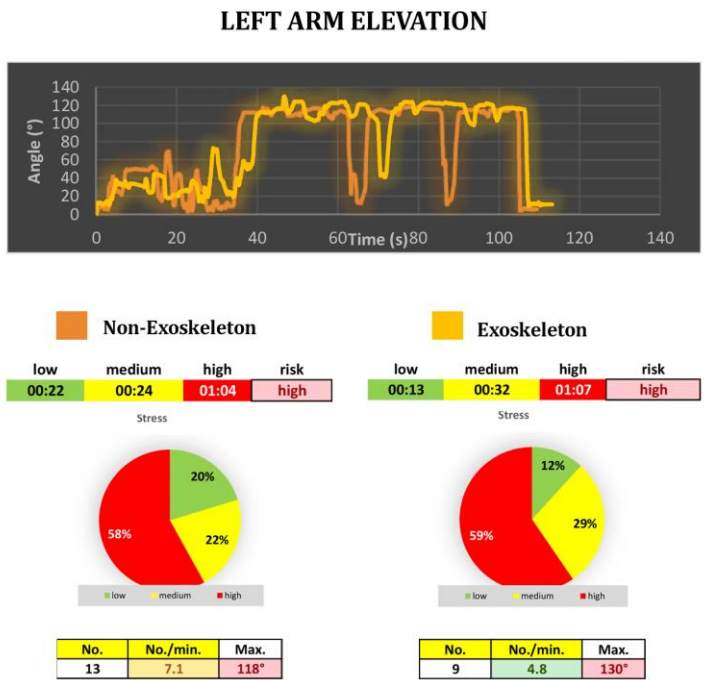
Figure 17. Left arm elevation results of Participant 7.
