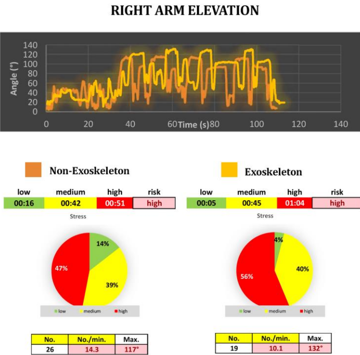
Figure 18. Right arm elevation results of Participant 7.
