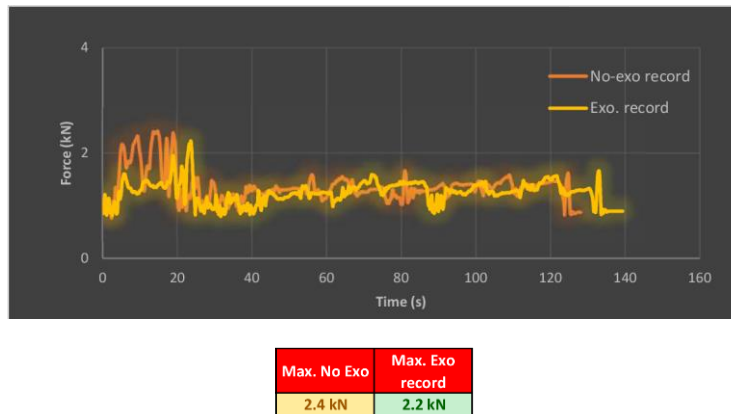
Figure 22. Comparison of the disc compression of participant 3.
