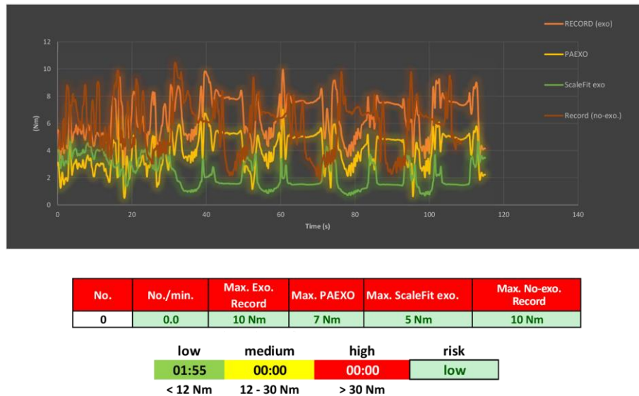
Figure 19. Participant 1 right shoulder moment comparison.
