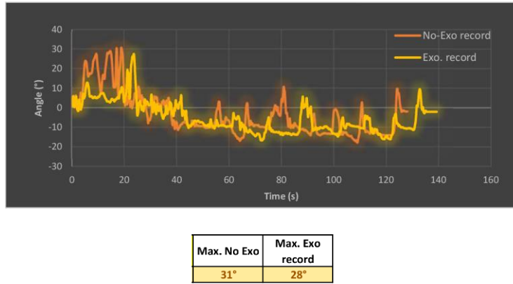
Figure 21. Trunk inclination comparison of participant 3.
