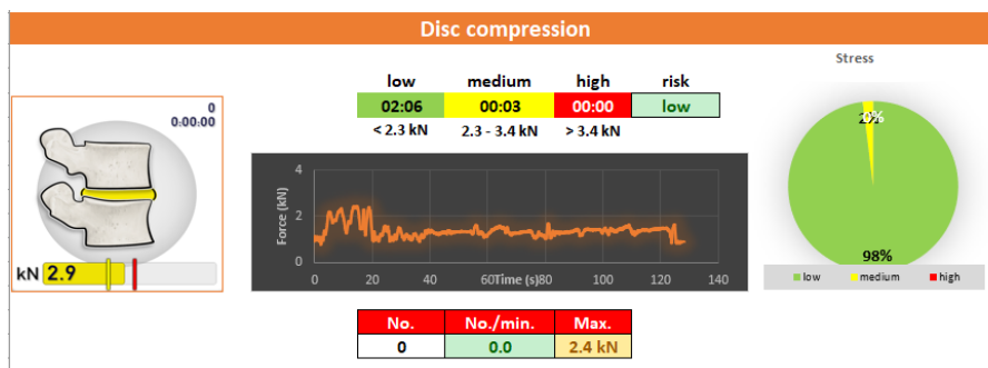
Figure 69. Disc compression graph of Participant 3 (Non-exoskeleton record).
