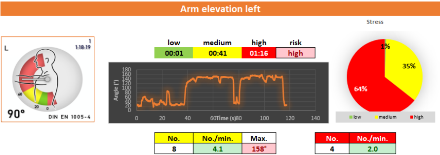
Figure 107. Left arm elevation graph of Participant 6 (Non-exoskeleton record).
