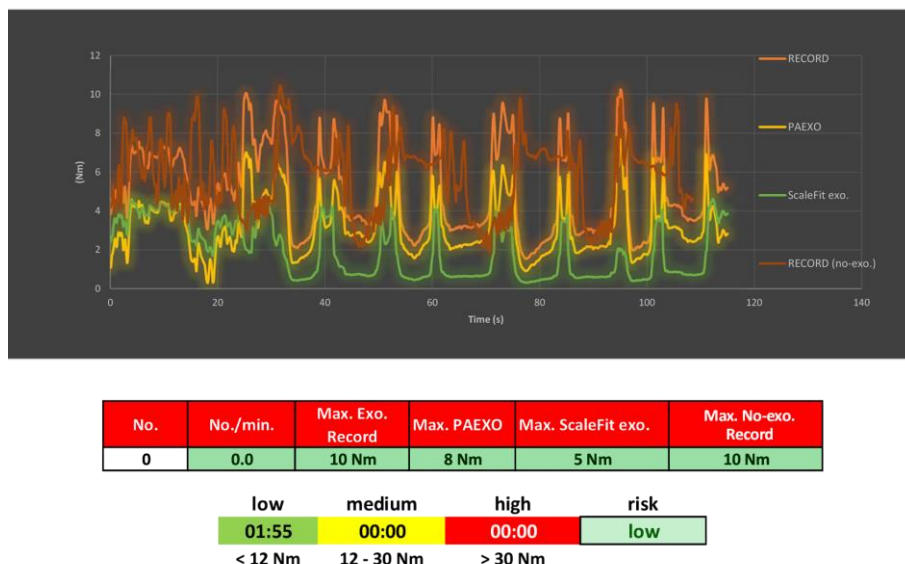
Figure 20. Participant 1 left shoulder moment comparison.
